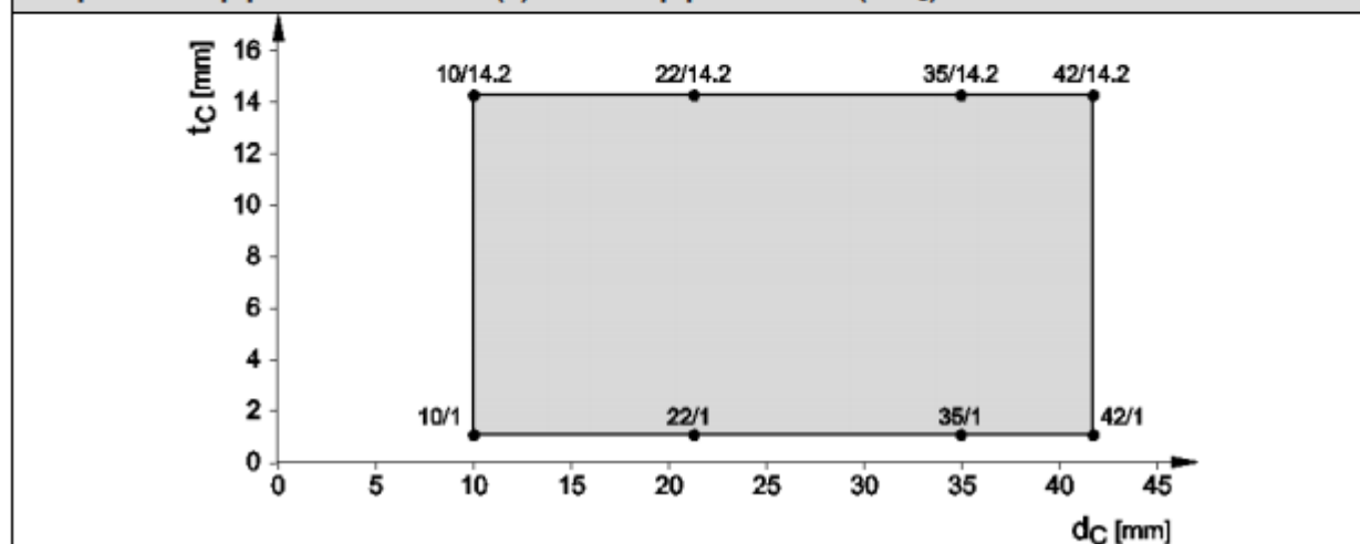
Copper pipe – relation wall thickness towards pipe diameter Graph shows pipe wall thickness (t c ) towards pipe diameter (Ø d c )
