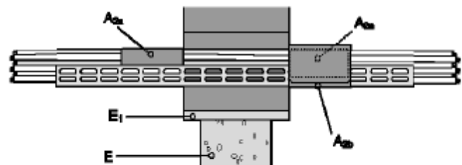
Figure 7: filler (A 1b ) plus 2 layers of putty, support tray
