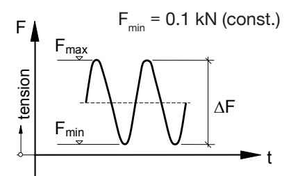
Principle sketch of cyclic tension tests
